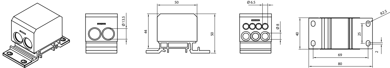
EDBM-8, EDBM-8/N, EDBM-8/PE - 70 mm 2
