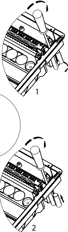
Holders for secure hollow wall installation
