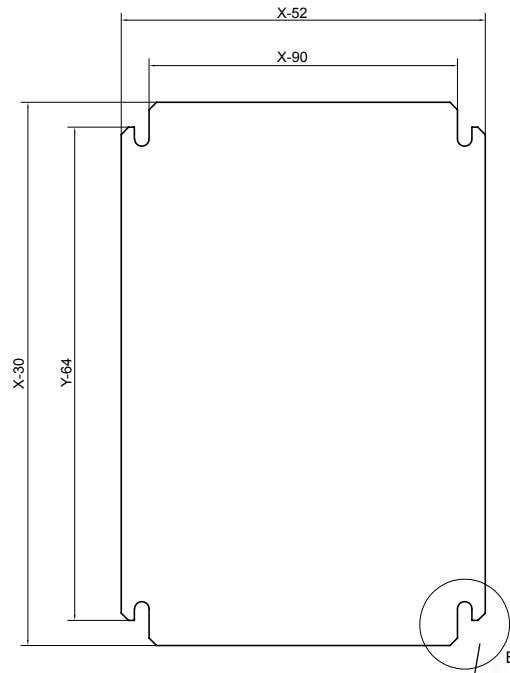
Mounting plate
